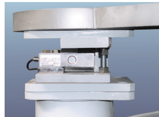
Fig.10 Load cell
